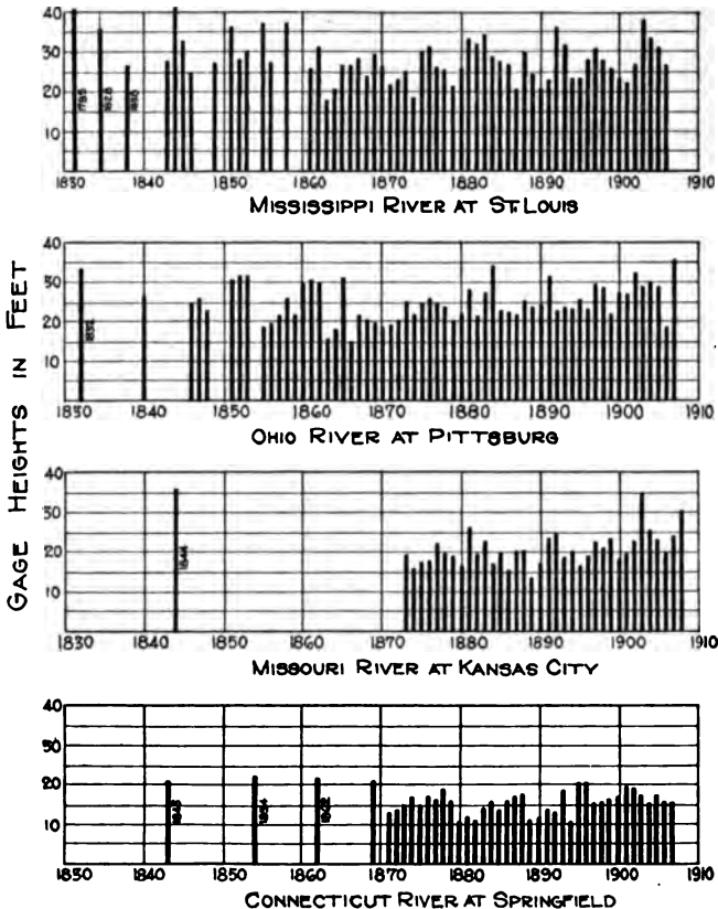
FIG. 8.—Long records of maximum annual high water.
